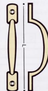
1436 SASH HANDLE lengths L : 102, 127, 152
